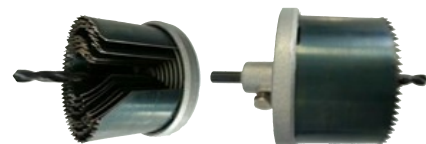
KW84-5070 (25, 32, 38, 45, 50, 56, 62 Ø) 2" 7 H. SIERRA 50 mm. ALTO
